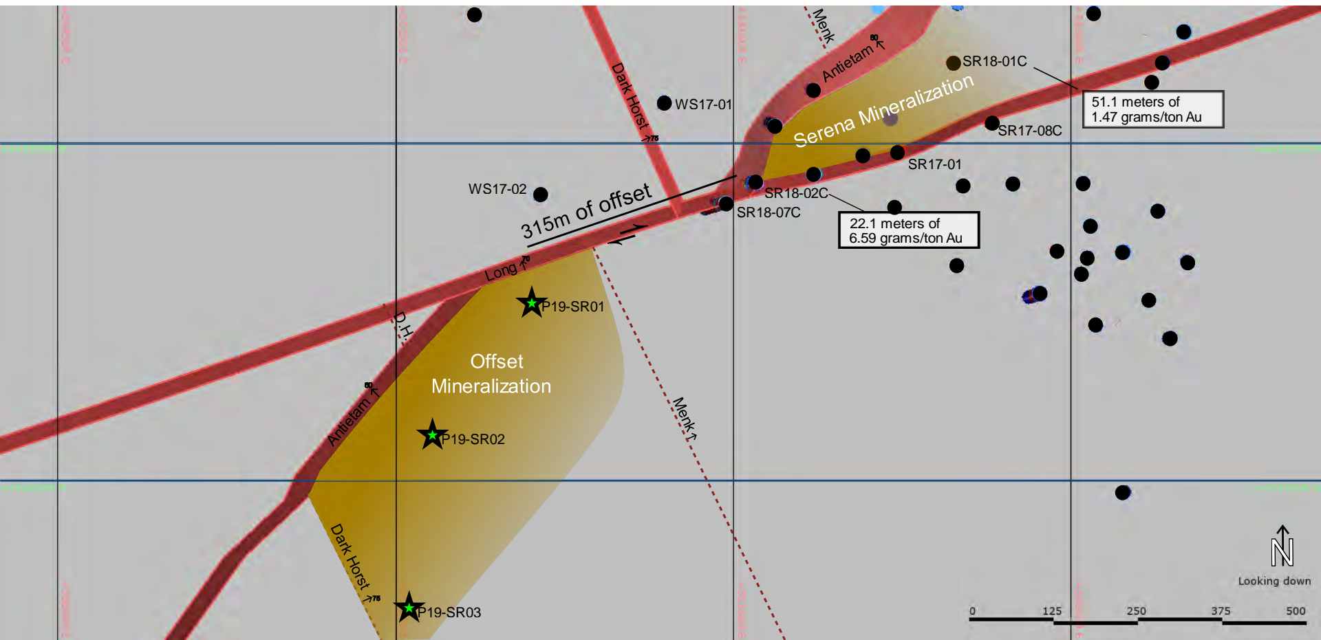
Serena Zone at 1650 meters elevation, (350 meter depth) showing anticipated right lateral offset of mineralized zone across Long Fault
